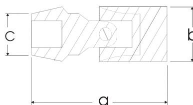
6 Point Universal Joint Sockets Standard Length
